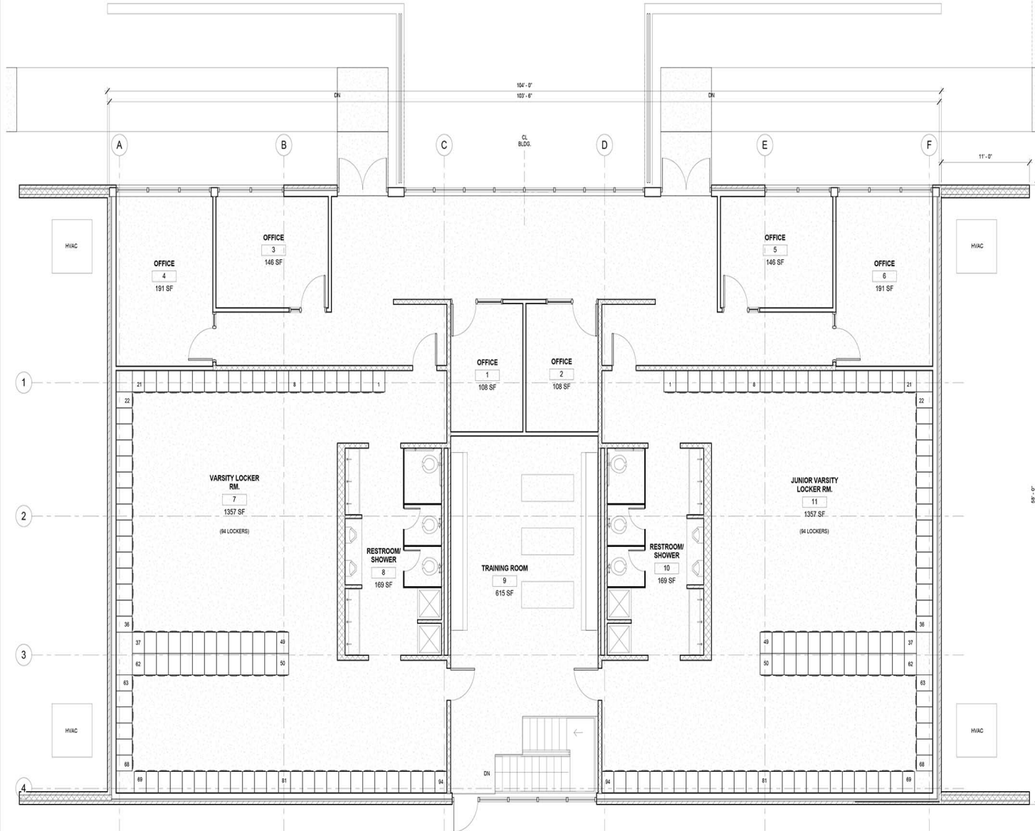
1 UPPER LEVEL FLOOR PLAN 1/4" = 1'-0"
